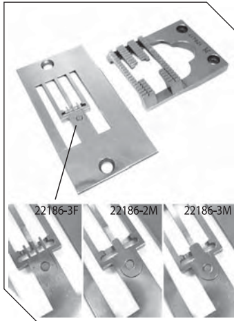
22186 針板 Needle Plate (連22186-3F 舌片) (with 22186-3F Supporting Finger)
