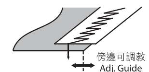
導帶坑面貼壓腳(附傍邊) Grooved Tape Attaching Foot with Guide
